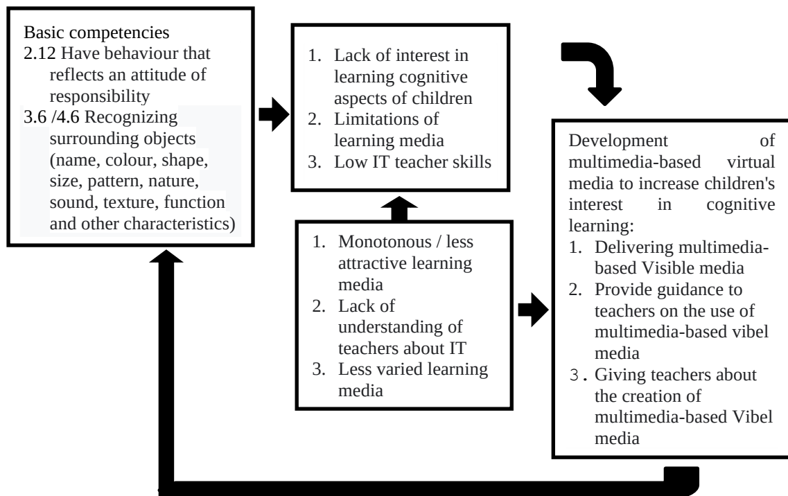
Figure 1. Thinking framework
